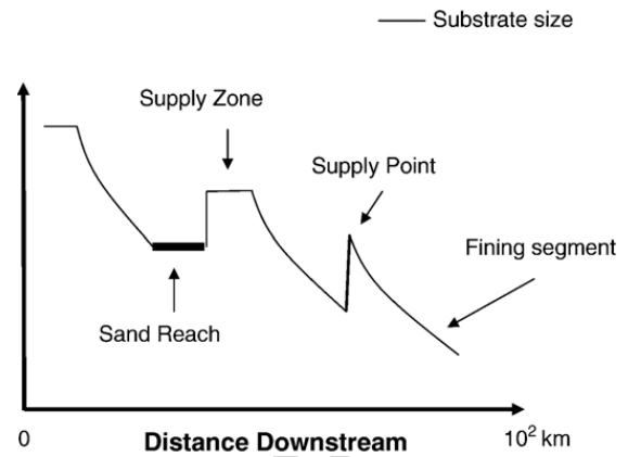
Fig. 11. Revised conceptual model of the sedimentary link incorporating two source types: local supply points and valley-segment supply zones.
